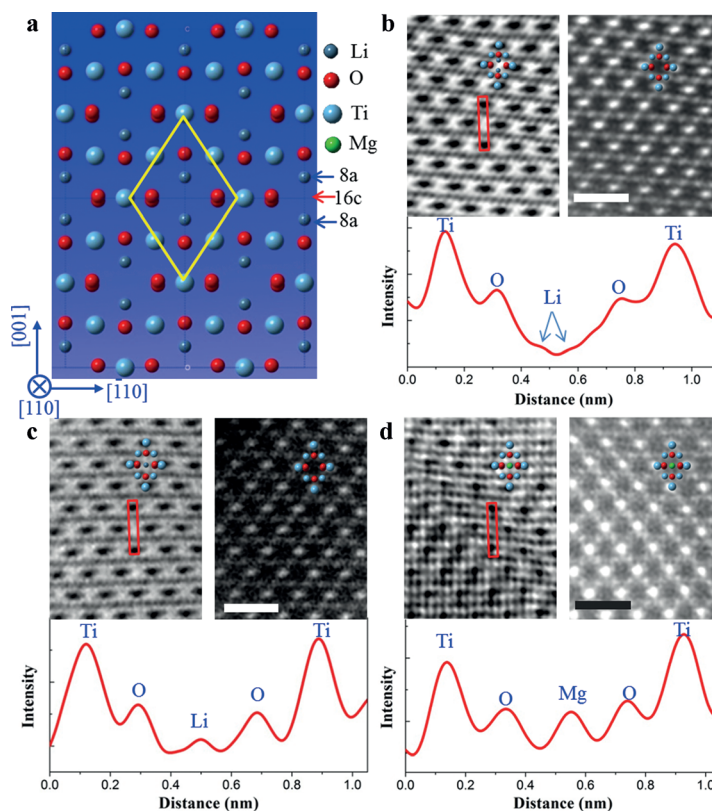
Figure 3. a) Schematic lattice of spinel Li4 viewed from the [110] zone axis, where the Ti, O, and Li columns are highlighted with light blue, red, and dark blue, respectively. b) HAADF, ABF images and ABF line profile for Li4 phase. c) The sample at the fully discharged state with the Li7 phase and d) Mg4Li phase. The Mg column is highlighted with green. Note that the image contrast of the dark dots is inverted and displayed as peaks in the ABF line profile. The scale bar equals 1 nm.
